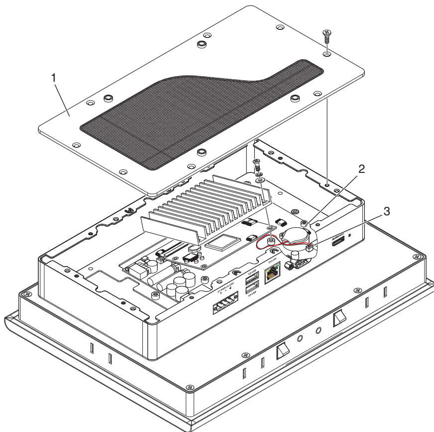
Figure 5-1 Battery replacement
