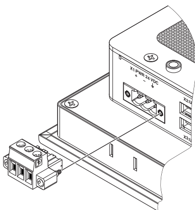
Figure 3-5 Power connection
